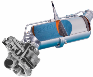
Particulate filter
