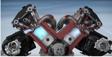
Cylinder deactivation
